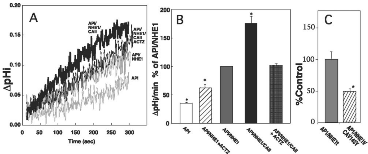
FIG. 4. Effects of CAII expression and acetazolamide on \text{H}^+ transport rate of AP1 cells in the presence of bicarbonate. Cell lines were initially bathed in \text{O}_2 bubbled HEPES-containing buffer ( \text{pH } 7.4 \pm 0.5 ) and then shifted to \text{CO}_2/\text{HCO}_3^- -containing buffer to create a bicarbonate-dependent acid load. The rate of recovery from an acid load was quantified as described earlier (27). A , examples of effects on intracellular pH. Representative effects on rate of recovery from an acid load induced by \text{CO}_2/\text{HCO}_3^- are illustrated. AP1 refers to AP1 cells that do not have an endogenous \text{Na}^+/\text{H}^+ exchanger. AP1/NHE1 refers to AP1 cells stably transfected with the plasmid pYN4+ that expresses the \text{Na}^+/\text{H}^+ exchanger (NHE1). AP1/pYN4+/CAII are AP1 cells stably transfected with NHE1 and the plasmid pJRC36 that expresses CAII. ACTZ indicates that the appropriate cells were treated with 100 \mu\text{M} acetazolamide. B , summary of \text{H}^+ transport rates of \text{Na}^+/\text{H}^+ exchanger and \text{Na}^+/\text{H}^+ exchanger and CAII-transfected cells. Results are mean \pm S.E. of at least seven experiments. Abbreviations are as in A . Asterisk indicates statistically significant difference from AP1/NHE1 cells at p < 0.05 . C , effect of dominant negative CAII with a V143Y mutation on \text{Na}^+/\text{H}^+ exchanger activity of AP1 cells. AP1 cells stably transfected with NHE1 were transiently transfected with either empty vector ( AP1/NHE1 ) or CAII with a V143Y mutation ( AP1/NHE1/CAIV143Y ). The activity of NHE1 was measured as described in the legend for Fig. 4. Results are mean \pm S.E. of four experiments.
