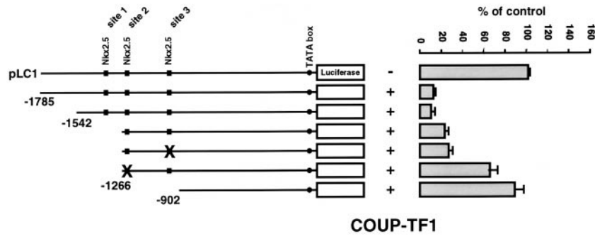
FIG. 3. Suppression by COUP-TF1 specifically requires the CRT site 2 in the calreticulin promoter. NIH3T3 cells were cotransfected with luciferase reporter constructs and with the COUP-TF1 expression vector. Luciferase activity was normalized against \beta -galactosidase. Three putative Nkx2.5 binding sites (CRT sites 1, 2, and 3) in the calreticulin promoter are indicated. X depicts deletion of a specific CRT site. Data are means \pm S.D. of three independent experiments.
